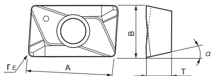
Fig.2 Peripheral Insert
