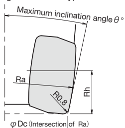
Fig.1 XPHW/T Type
