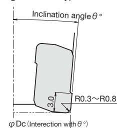
Fig.2 YPHW Type
