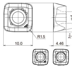
Fig.4 SPMT100415ZPTR-PM
