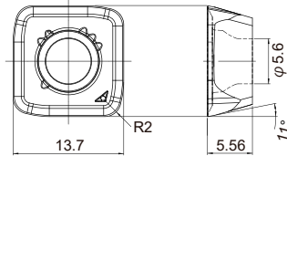
Fig.2 SPMT140520ZPER-SM
