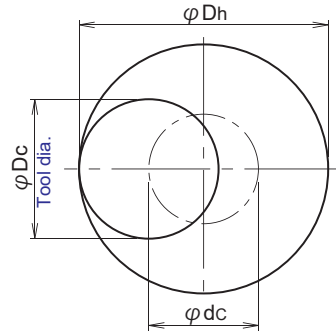
Helical interpolation
