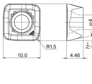
Fig.3 SPMT100415ZPER-SM
