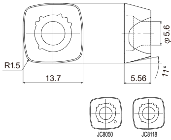
Fig.1 SPNW140515ZTR
