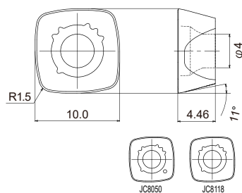
Fig.1 SPNW100415ZTR
