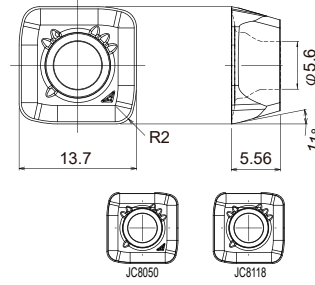
Fig.3 SPMT140520ZPTR-PM
