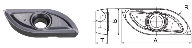
Fig.4 (Sub blade for welding & hardened material)
